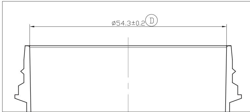
NECK DETAIL SCALE 2
