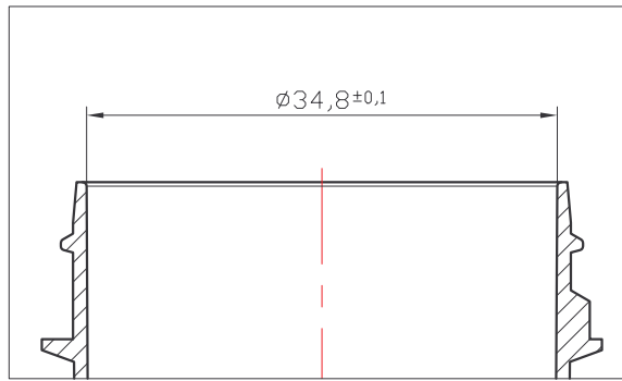
NECK DETAIL SCALE 2
